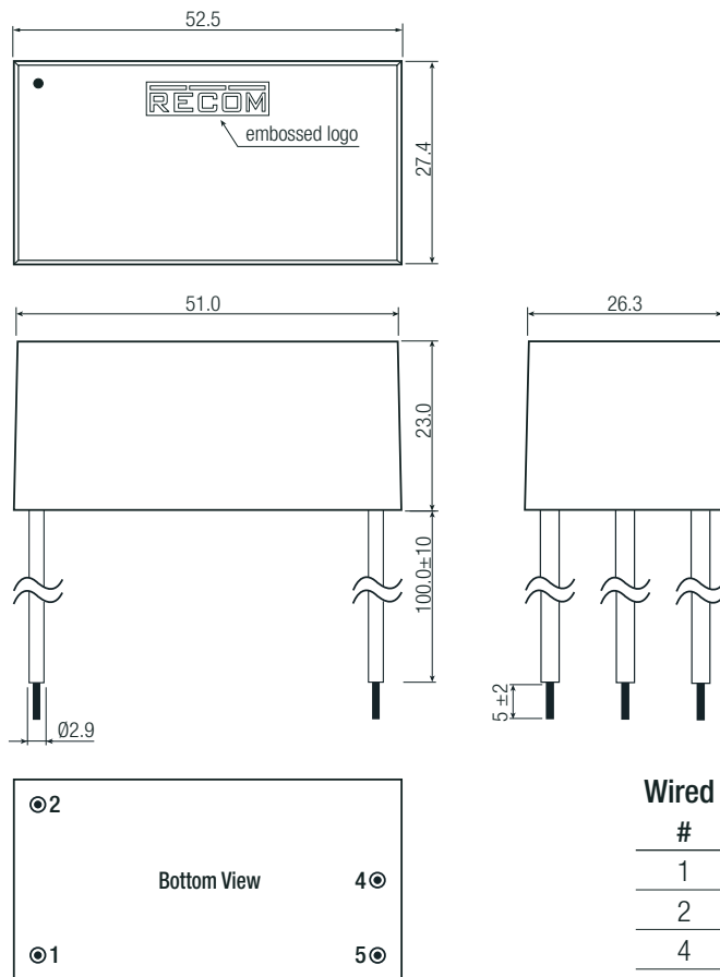
Dimension Drawing Single Wired (mm)
